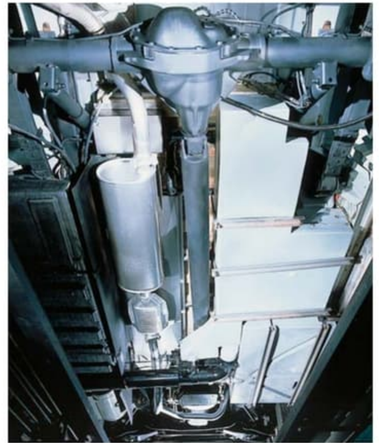
Water tanks fit below the floor which maximizes interior storage space. Locating them between the axles improves weight distribution for better handling.
