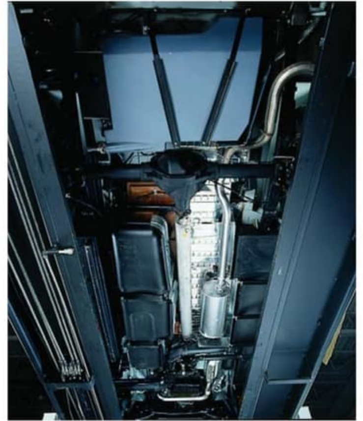
Water tanks fit below the floor which maximizes interior storage space and improves weight distribution for better handling.
