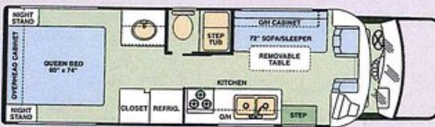
Model C290: Rear Bedroom, Queen Walkaround Bed, Side Dinette Optional Water Tank Capacities (gallons): Black: 32 • Gray: 26 • Fresh: 30
