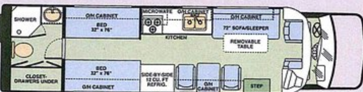
Model 312SD (Ford only): Large Rear Bath, Twin Beds, Side Dinette Water Tank Capacities (gallons): Black: 32 • Gray: 26 • Fresh: 31 Floor plans, features and specifications of the ISATA are subject to change without notice.
