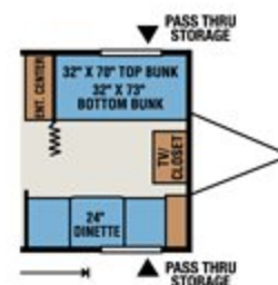
S330BH Bunk/Dinette Option
