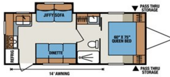
S241RKS • Twin Beds Option – see below
