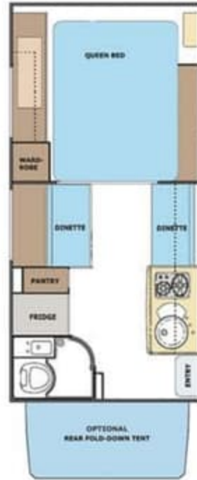
830 8'11" SHORT BED TRUCK
