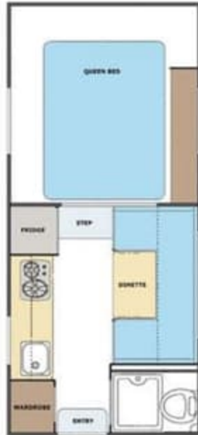
825 8'6" SHORT BED TRUCK
