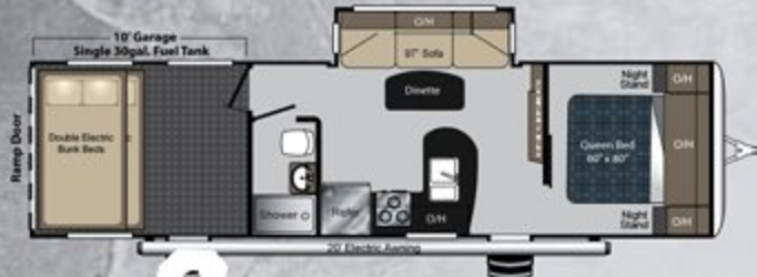
32 TRAVEL TRAILER SHIPPING WEIGHT: 8,450 LBS HITCH WEIGHT: 1,275 LBS LENGTH: 35' 5"
