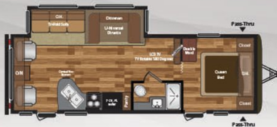
WEIGHT: 6125 LENGTH: 29' 11" 26RLSWE
