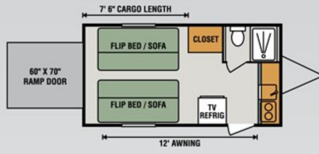
140TH Toy Hauler
