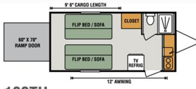
160TH Toy Hauler
