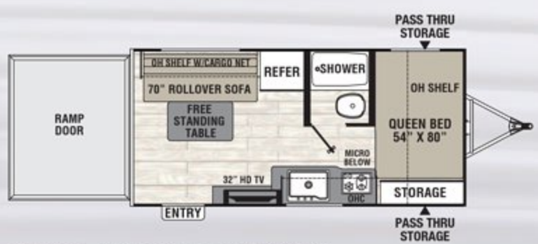
17 BLSE / Exterior Length 20' 4"
