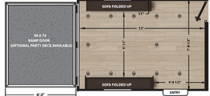
29THS GARAGE DIMENSIONS
