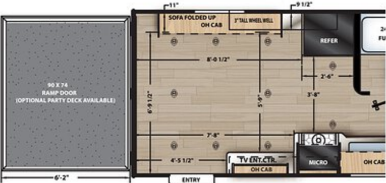
19TH GARAGE DIMENSIONS
