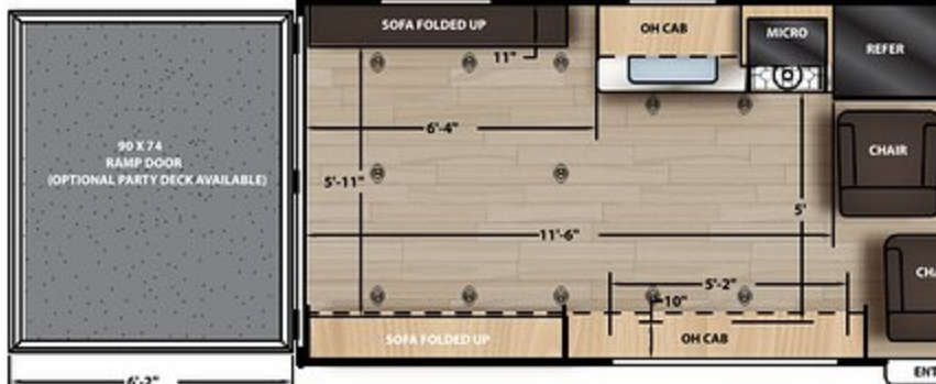
26TH GARAGE DIMENSIONS
