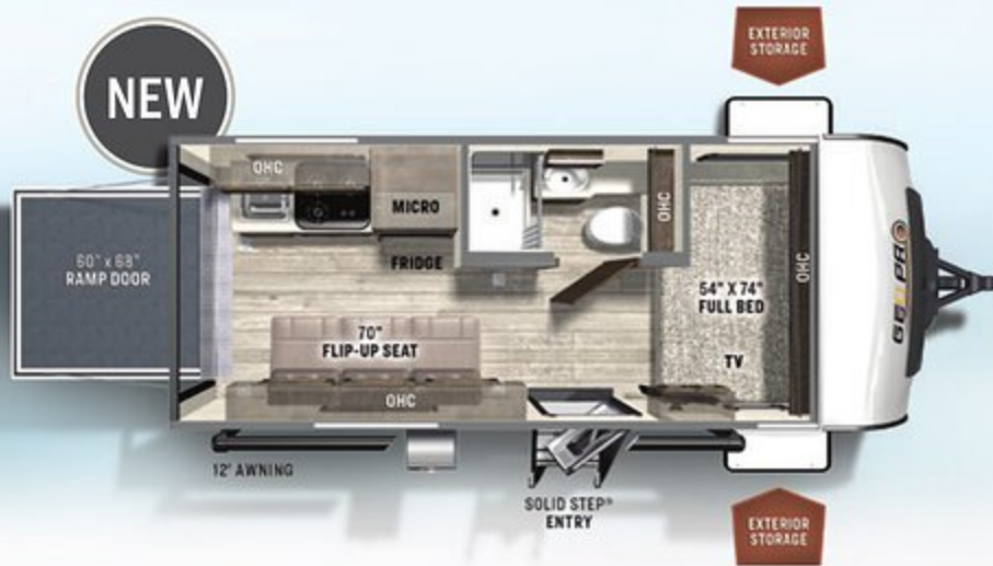
19FBTH TOY HAULER UUV: 3873 HITCH: 620 AXLE: 3215 CCC: 1097 LENGTH: 20' 2" WIDTH: 7' 8" GEO PRO HEIGHT: 10' INT. HEIGHT: 6' 6" FRESH: 31 gal GRAY: 16 gal BLACK: 30 gal
