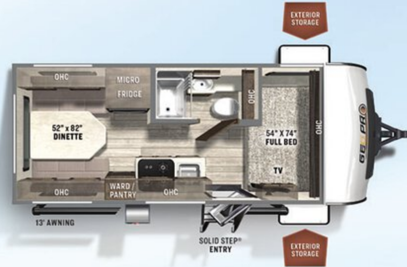
19RD REAR DINETTE UUV: 3271 HITCH: 436 AXLE: 2797 CCC: 1065 LENGTH: 20' 2" WIDTH: 7' 8" GEO PRO HEIGHT: 9' 10" INT. HEIGHT: 6' 6" FRESH: 31 gal GRAY: 30 gal BLACK: 30 gal
