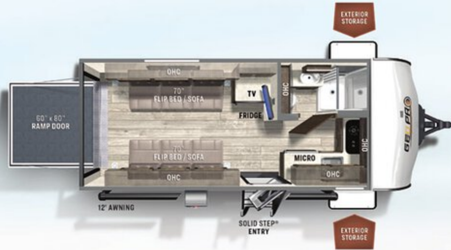
19TH TOY HAULER UUV: 3407 HITCH: 641 AXLE: 2728 CCC: 1584 LENGTH: 20' 2" WIDTH: 7' 8" GEO PRO HEIGHT: 10' INT. HEIGHT: 6' 6" FRESH: 31 gal GRAY: 16 gal BLACK: 30 gal
