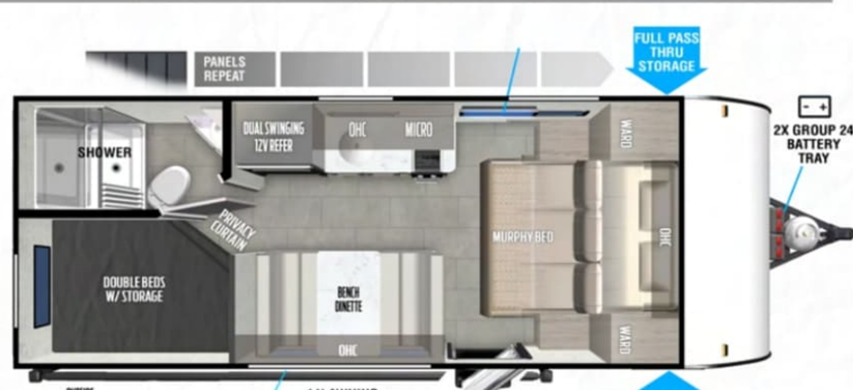
14' AWNING 179DBK LENGTH: 22' 6" UVW: 3,829 LBS
