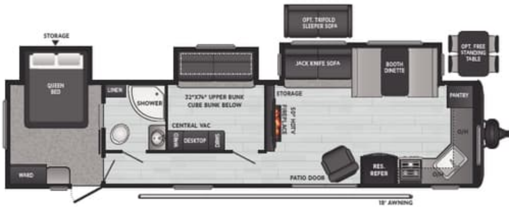
38FK | WEIGHT 9183 | LENGTH 39' 11"
