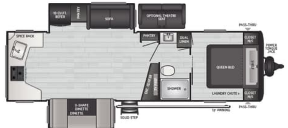
281RK | WEIGHT TBD | LENGTH 32' 5"
