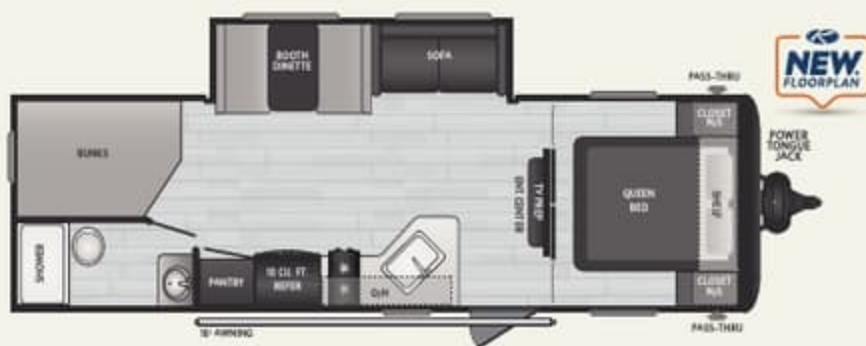
261BHC | WEIGHT 6115 | LENGTH 30' 8"
