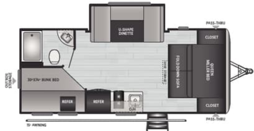
1810BH | WEIGHT 4405 | LENGTH 20' 6"
