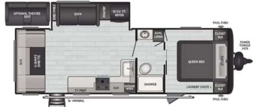
256RD | WEIGHT 6383 | LENGTH 29' 11"
