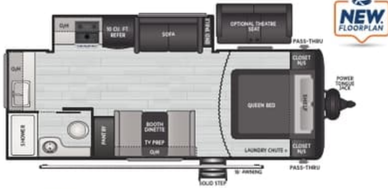
220ML | WEIGHT 5645 | LENGTH 26' 2"
