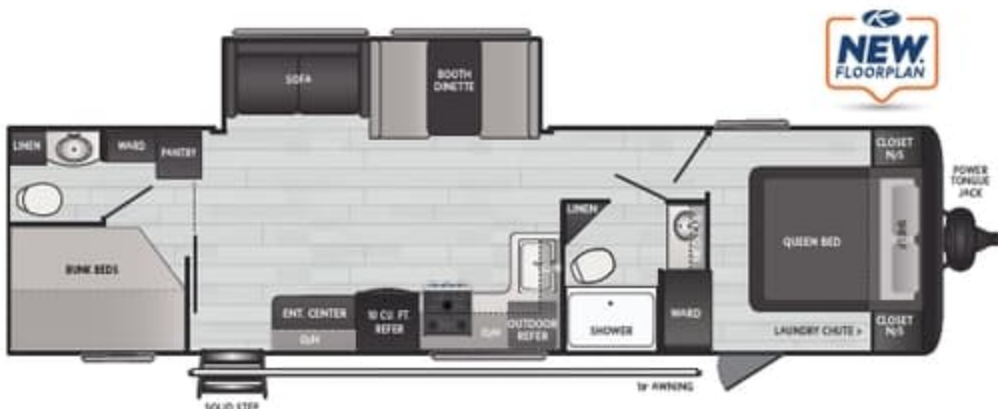
310DB | WEIGHT 7640 | LENGTH 35' 11"
