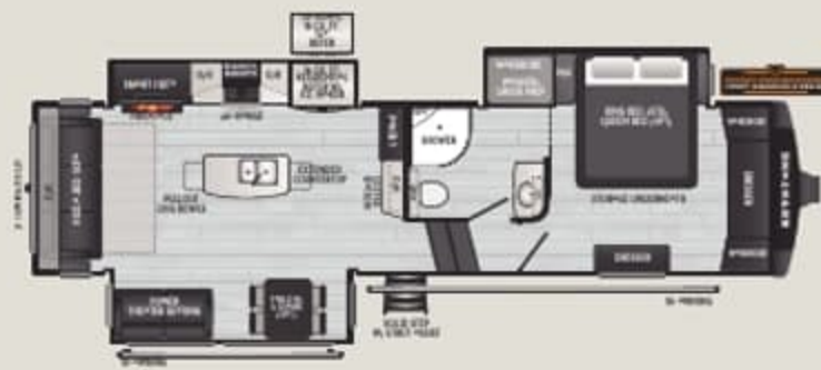
295RL | WEIGHT 11692 | LENGTH 34' 0"
