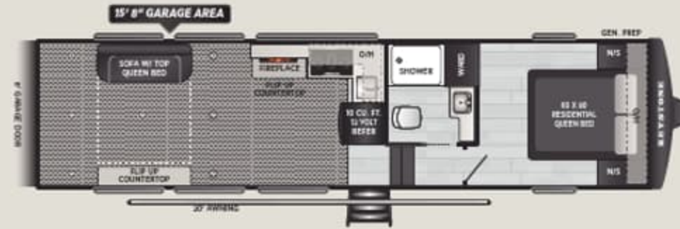
321LT WEIGHT 9320 LENGTH 32' 0"
